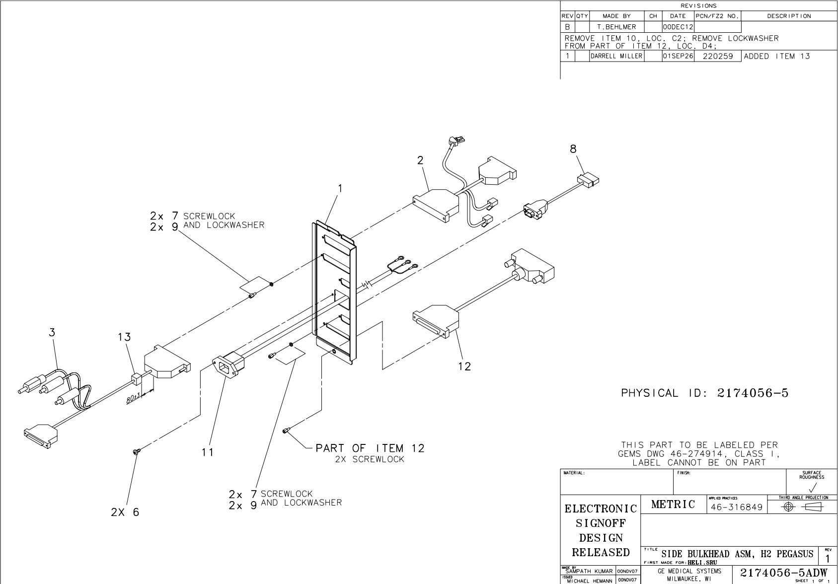
Figure 5-35 Bulkhead Assembly, Side (2174056-5, sheet 1, rev 1)
