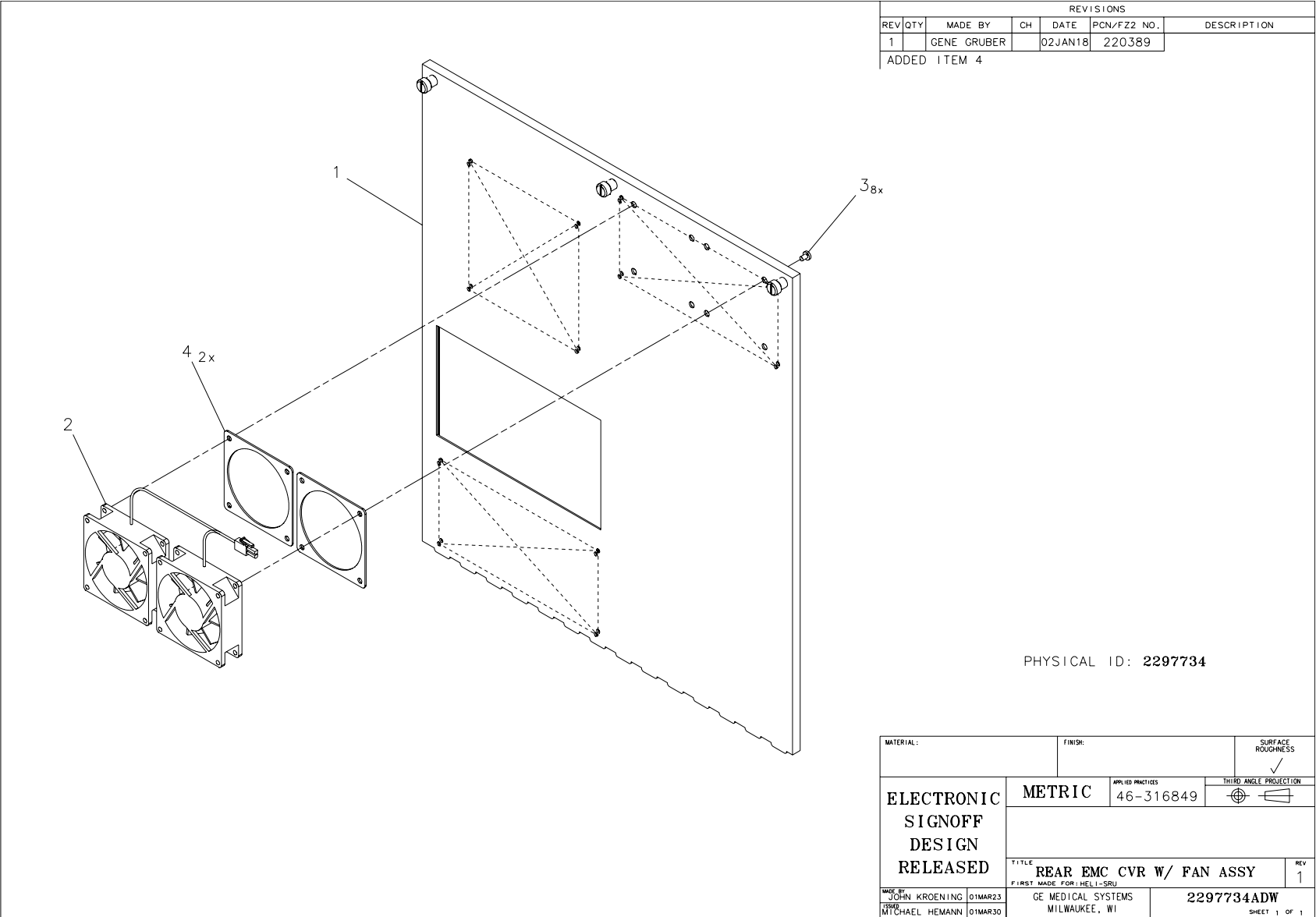
Figure 5-22 Rear Cover w/Fan (2297734, sheet 1, rev 1)
