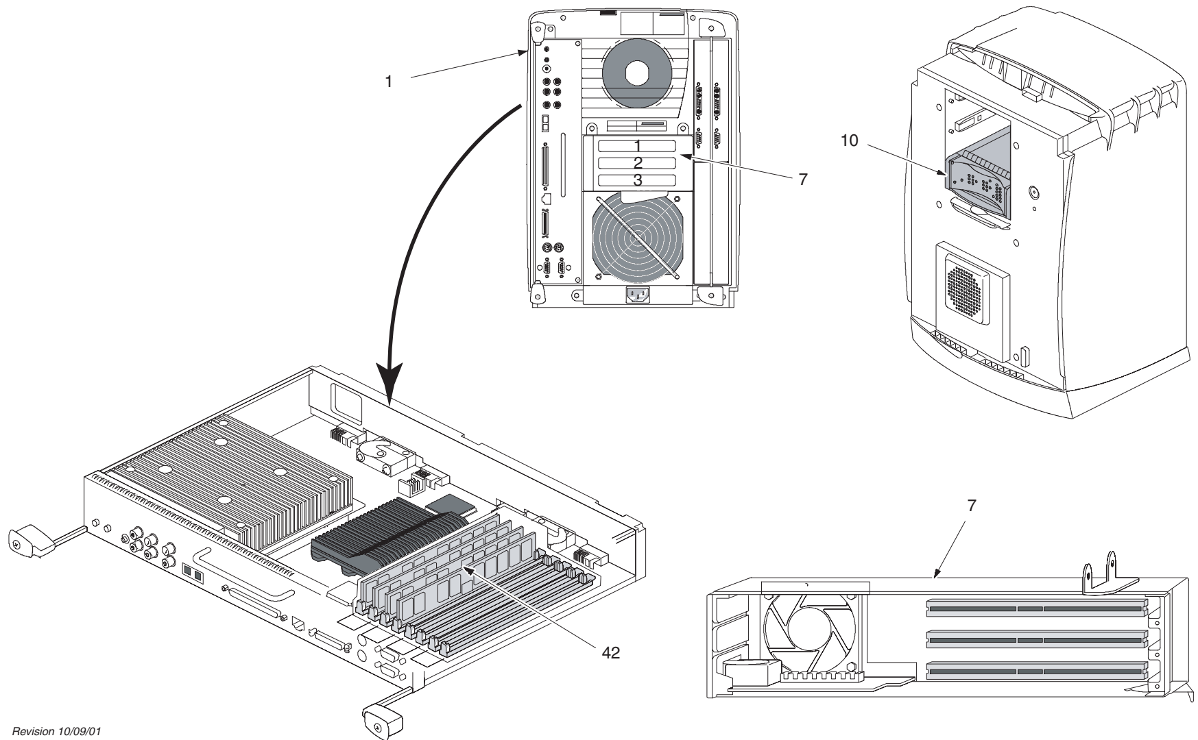
Figure 5-21 Octane2 Replacement Parts (sheet 1, rev 10/09/01)
