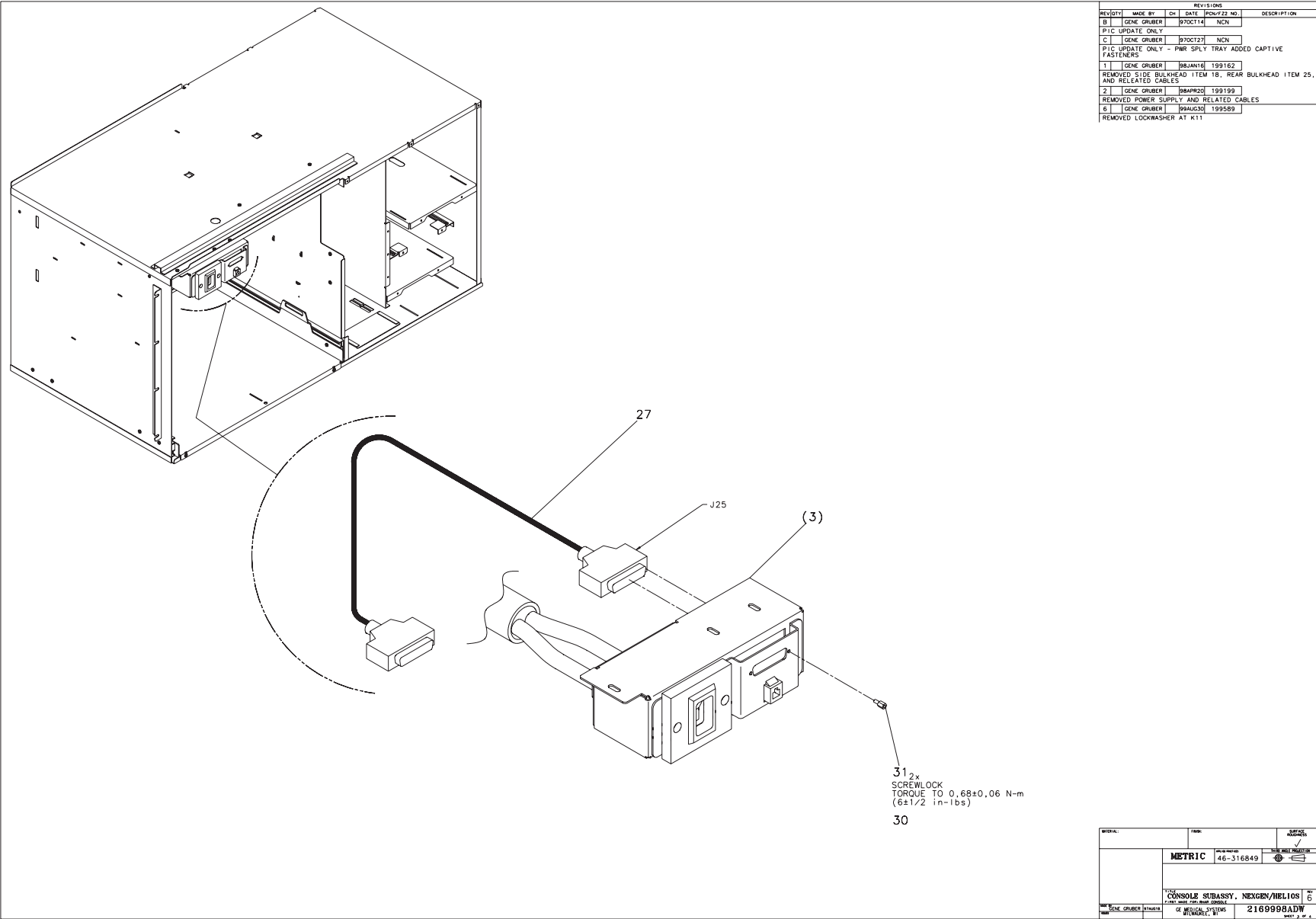
Figure 5-25 Nexgen/Helios Console Sub-Assy (2169998, sheet 3, rev 6)
