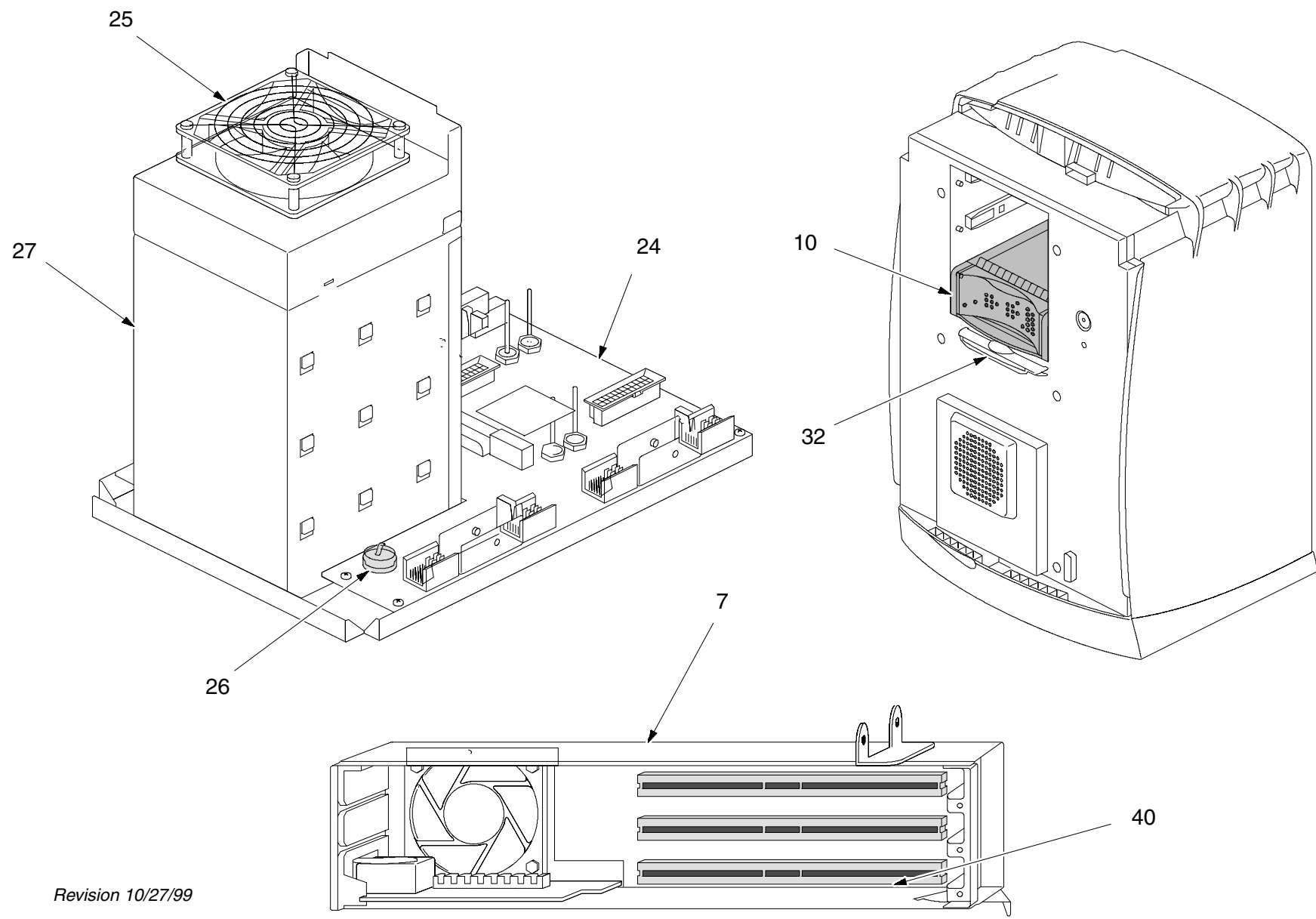
Figure 5-19 Octane Computer, (sheet 2, rev 10/27/99)
