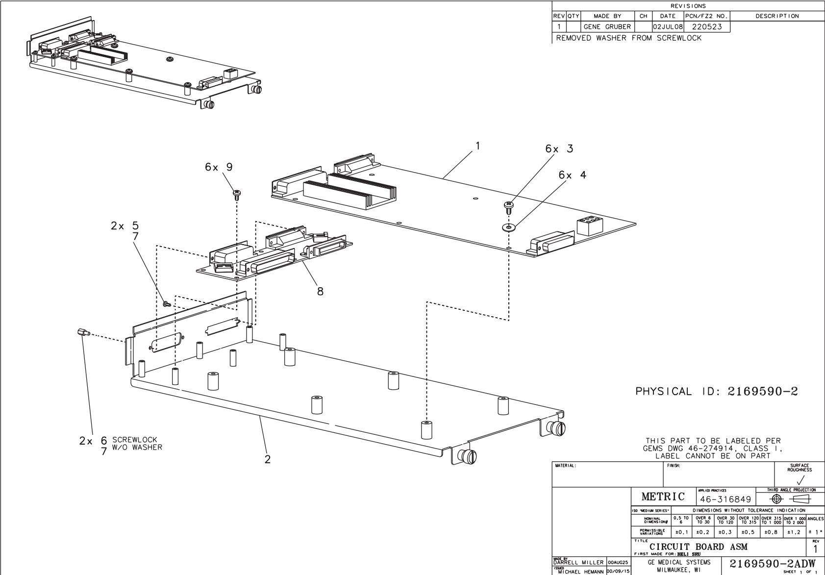
Figure 5-33 CR Intercom/Prescribed Tilt Circuit (2169590-2, sheet 1, rev 1)
