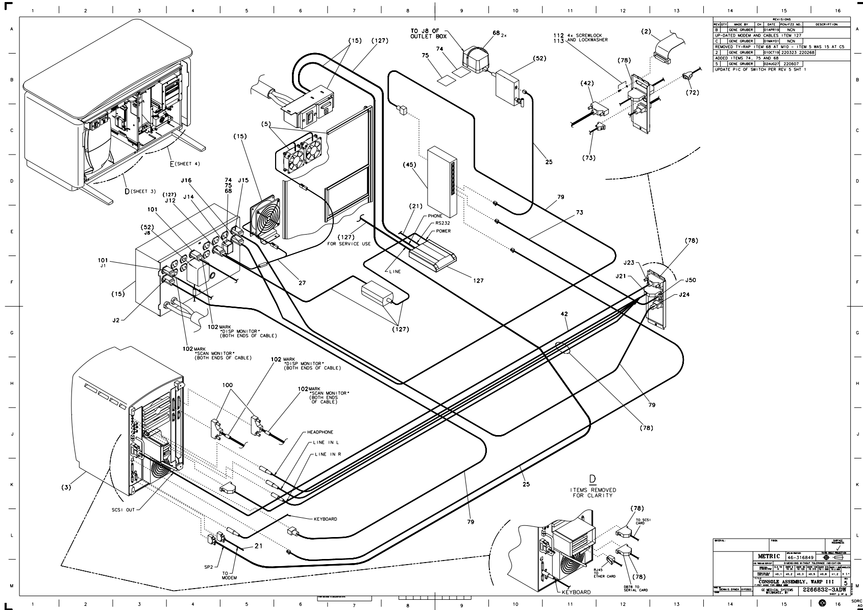
Figure 5-4 Console Assembly (2266832-3, sheet 3, rev 5)
