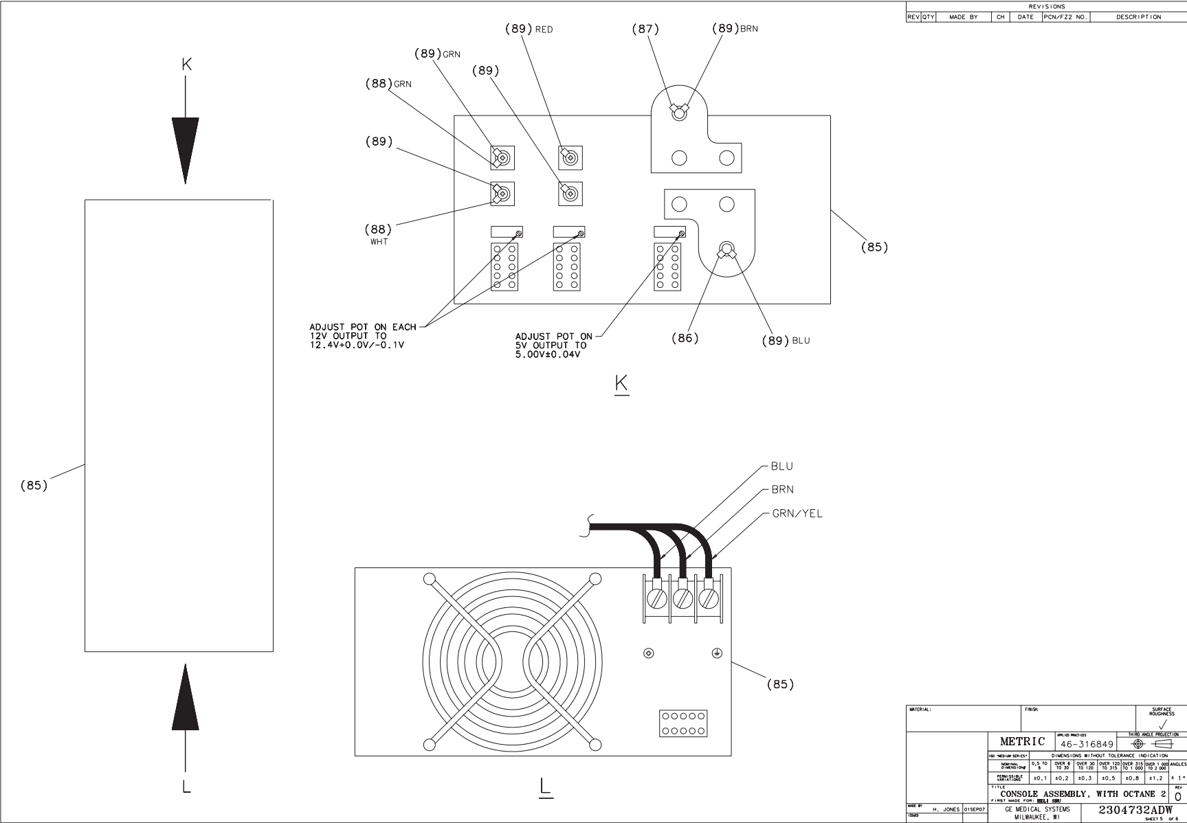
Figure 5-12 Console Assembly, w/Octane2 (2304732, sheet 5, rev 0)
