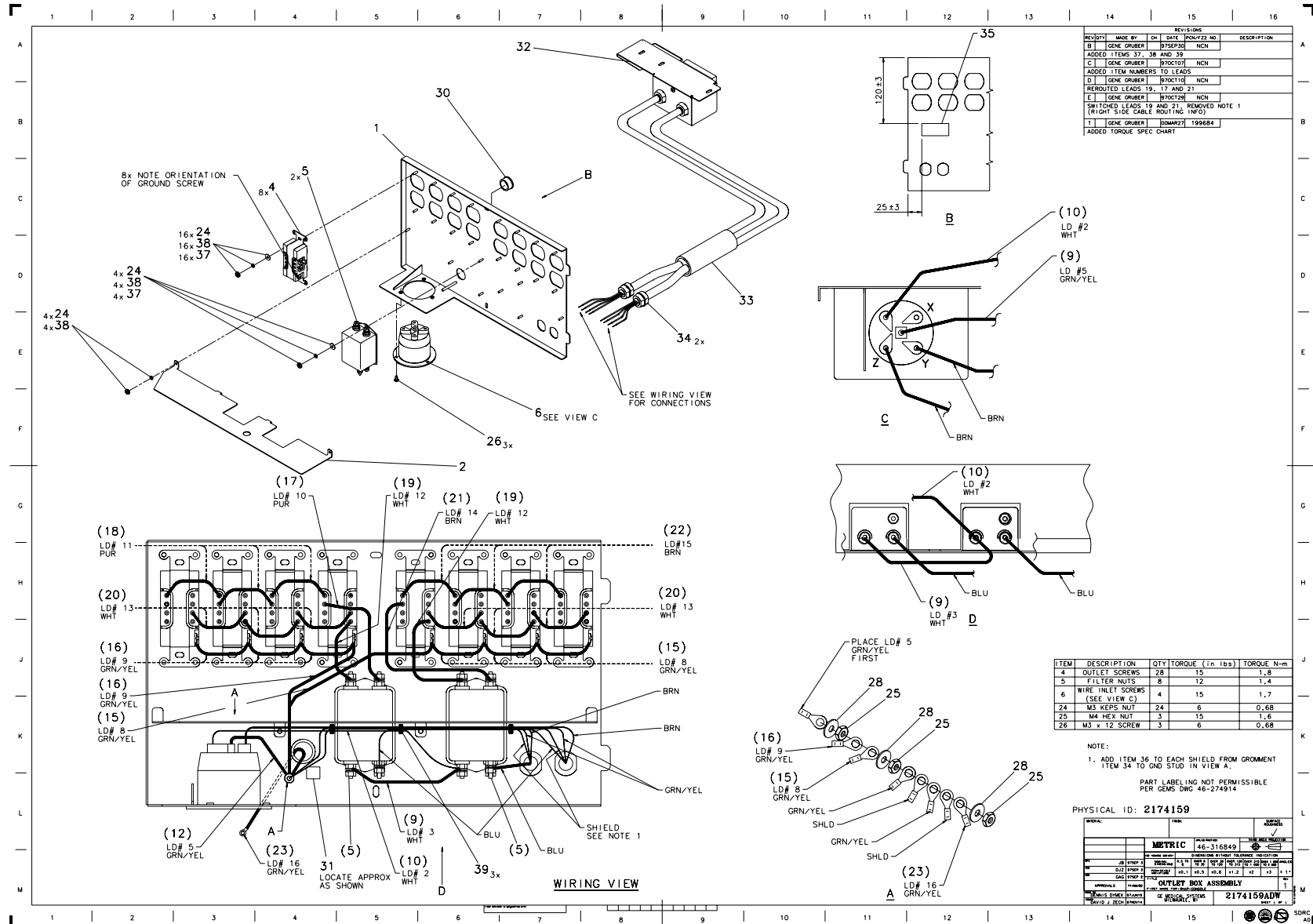
Figure 5-29 Outlet Box Assembly (2174159, sheet 1, rev 1)
