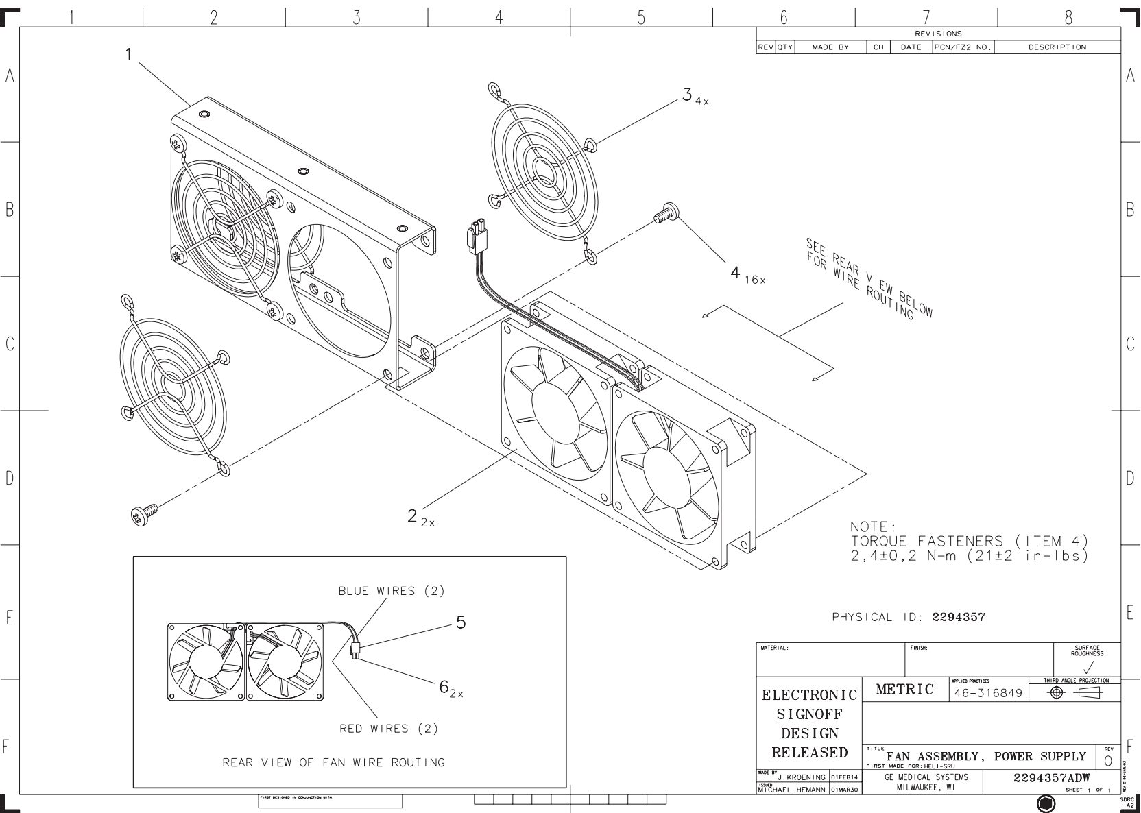
Figure 5-34 Box Assy - Fan and Cables (2294357, sheet 1, rev 0)
