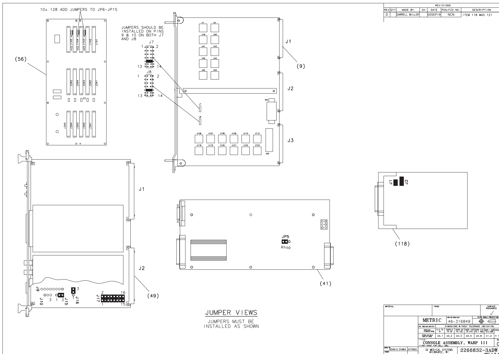
Figure 5-7 Console Assembly (2266832-3, sheet 6, rev 0)
