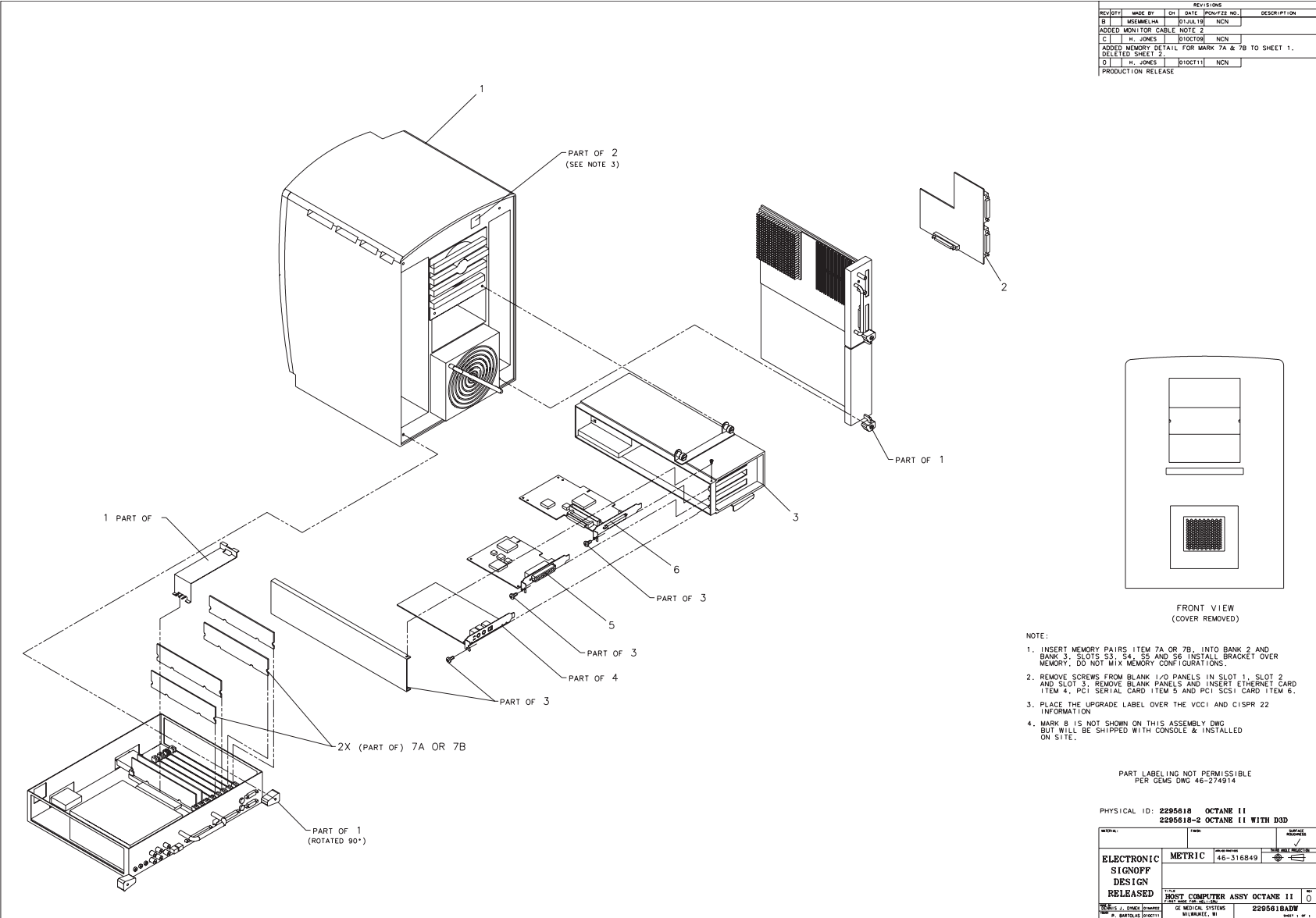
Figure 5-20 Octane2 Computer Assembly (2295618, sheet 1, rev 0)
