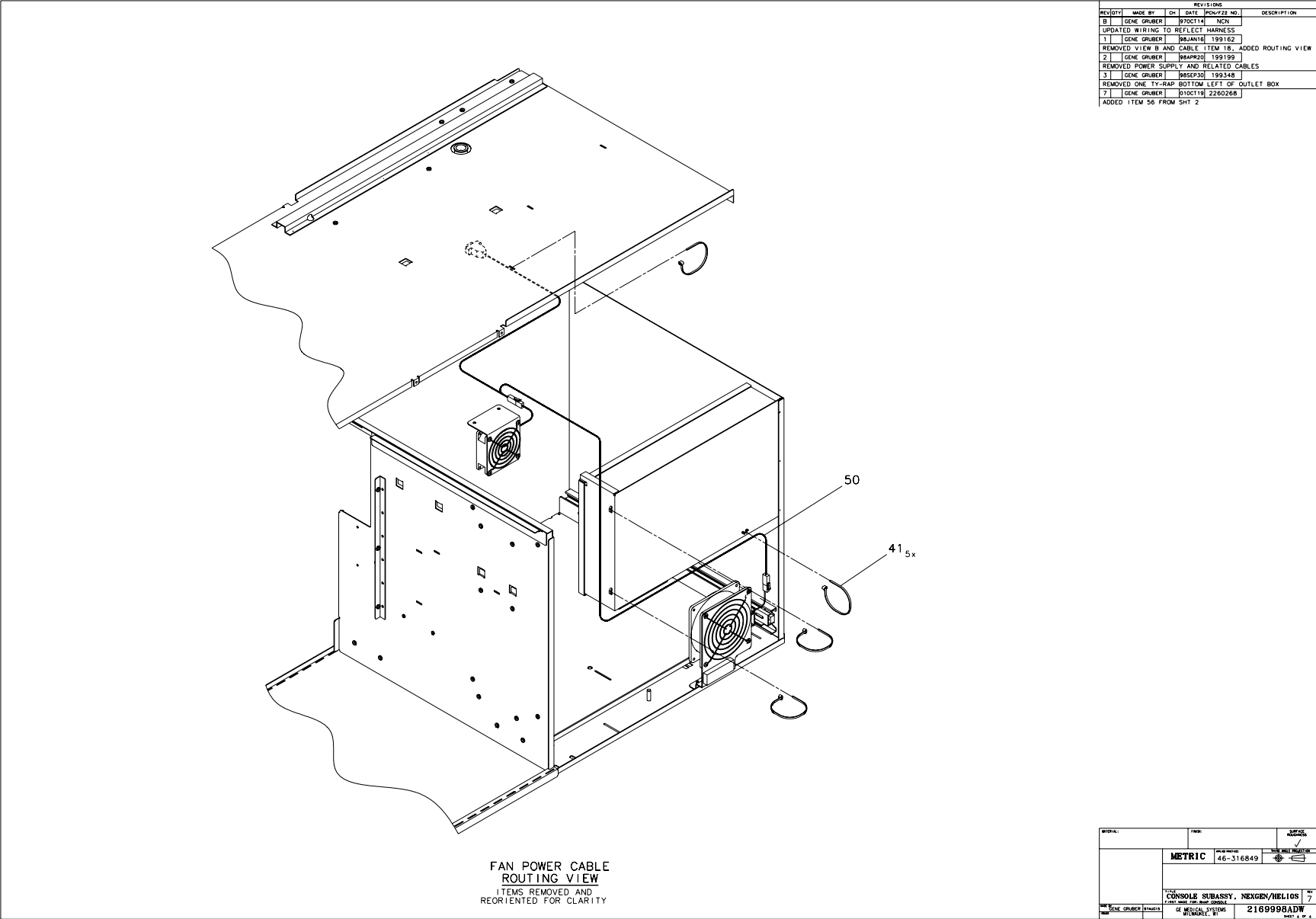
Figure 5-26 Nexgen/Helios Console Sub-Assy (2169998, sheet 4, rev 7)
