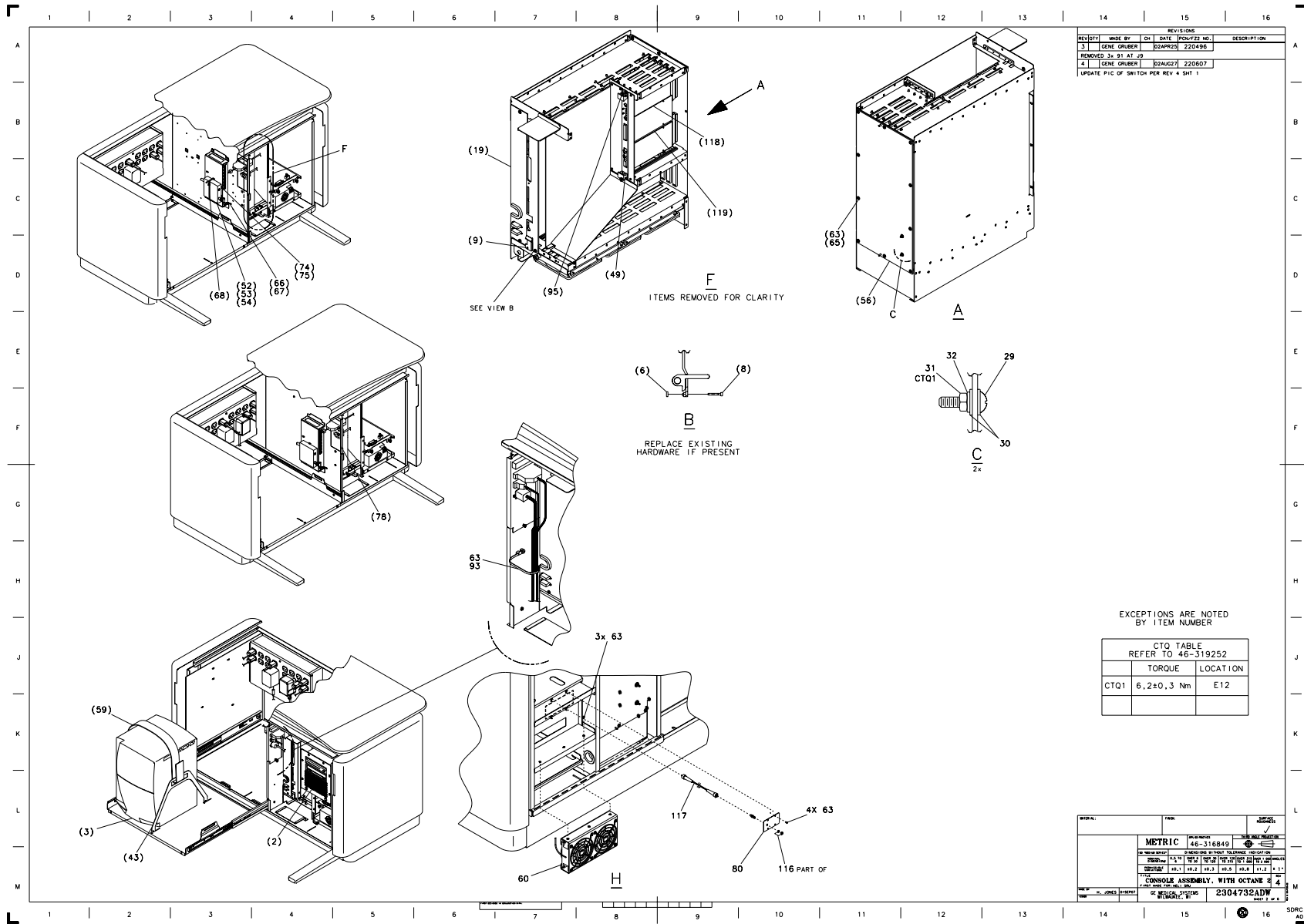
Figure 5-9 Console Assembly, w/Octane2 (2304732, sheet 2, rev 4)
