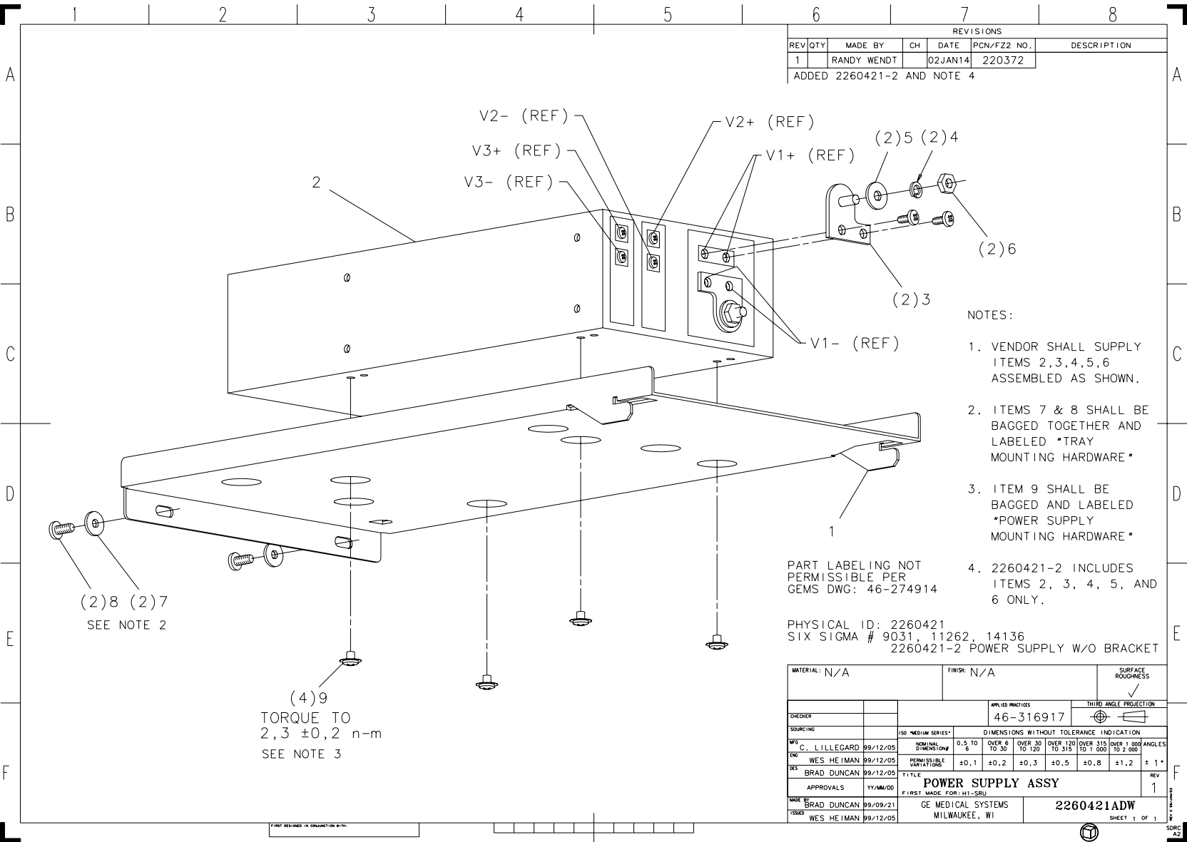
Figure 5-36 VME Console Power Supply Assembly (2260421, sheet 1, rev 1)
