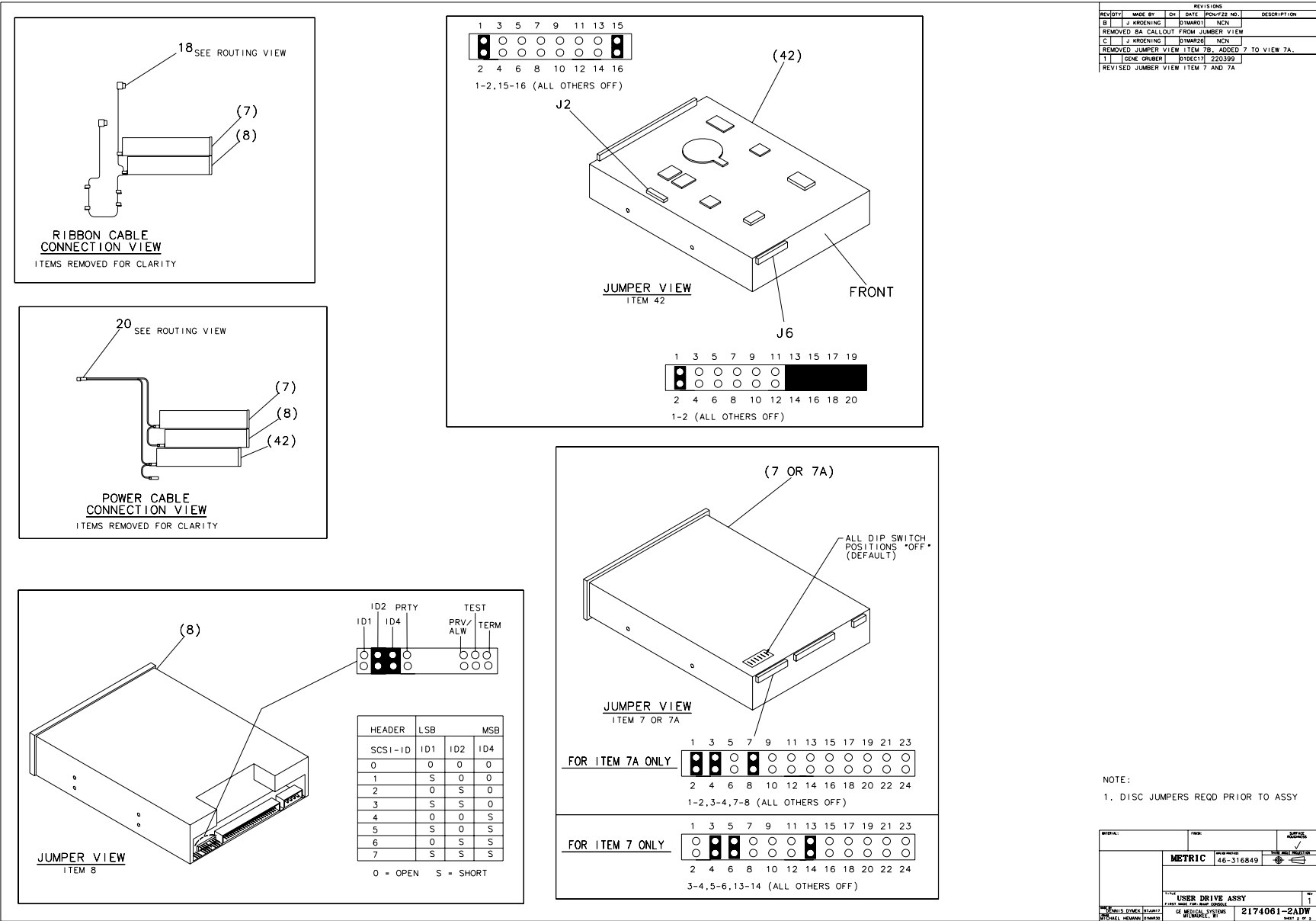
Figure 5-15 Console User Drive Assembly (2174061-2, sheet 2, rev 1)
