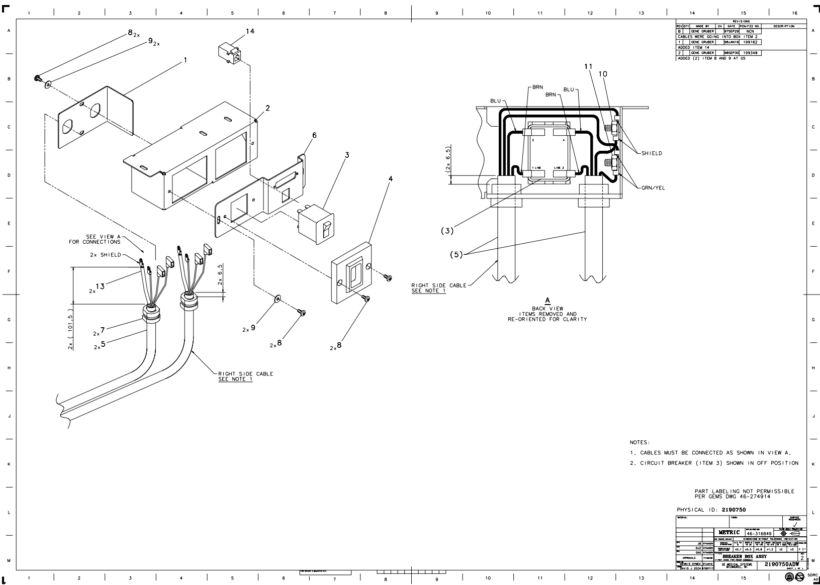
Figure 5-30 Breaker Box Assembly (2190750, Sheet 1, rev 2)
