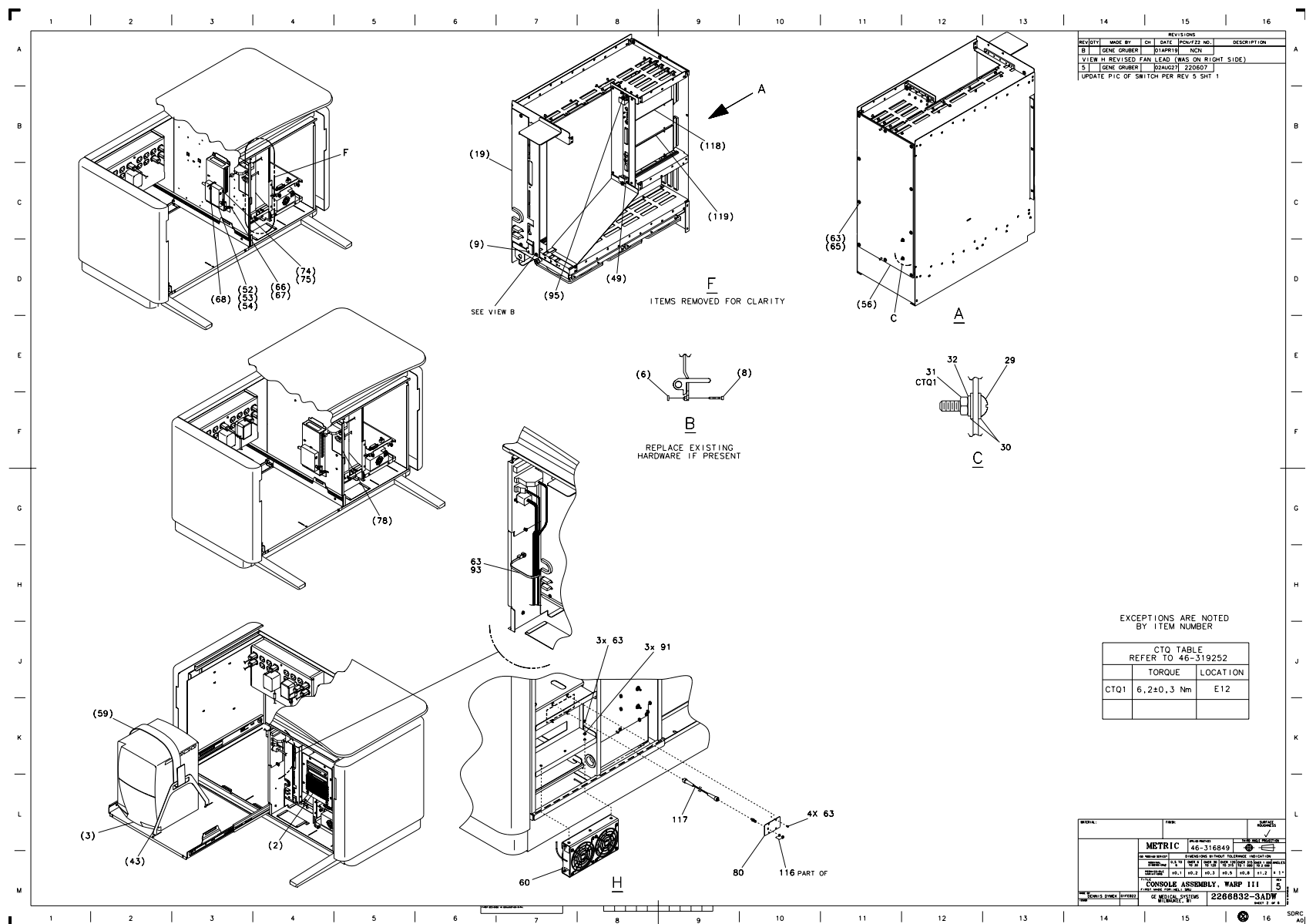
Figure 5-3 Console Assembly (2266832-3, sheet 2, rev 5)
