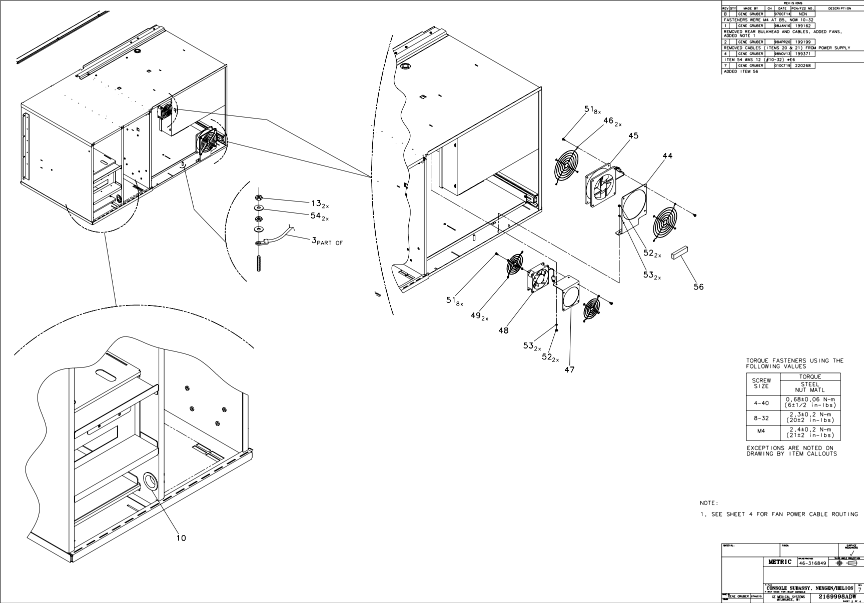
Figure 5-24 Nexgen/Helios Console Sub-Assy (2169998, sheet 2, rev 7)
