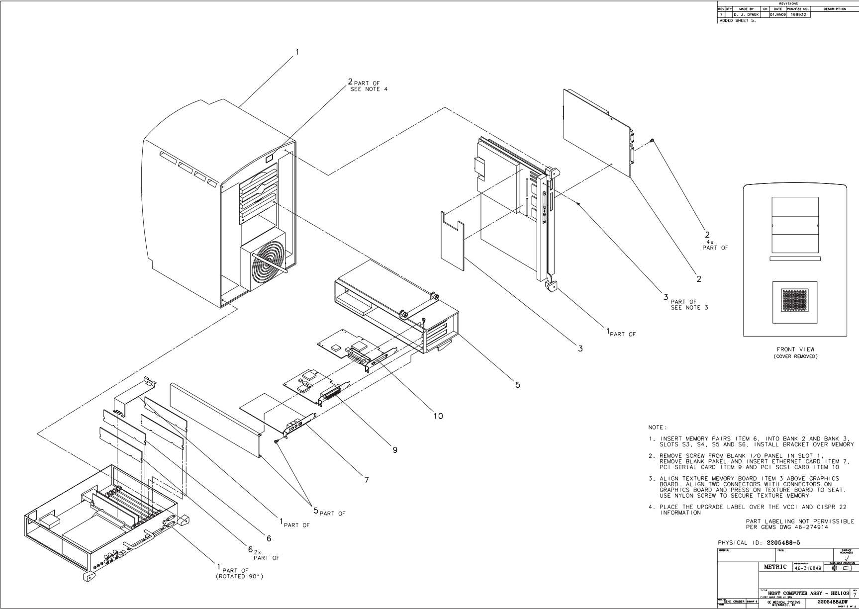
Figure 5-17 Octane Computer Assembly w/D3D (2205488, sheet 5, rev 7)
